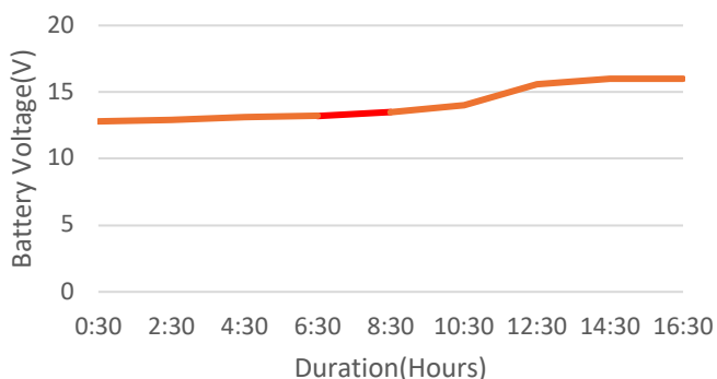
Charge Characteristics Graph
