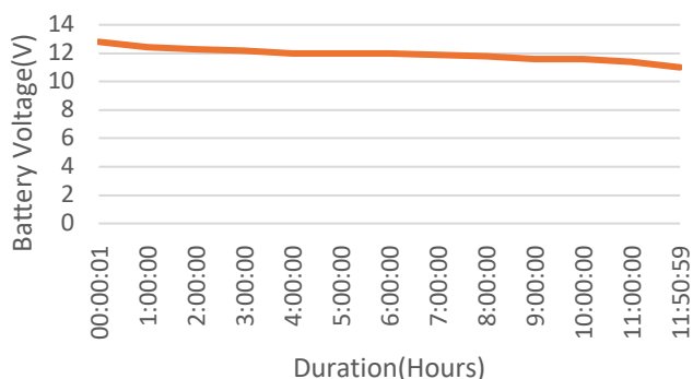
Discharge Characteristics Graph
