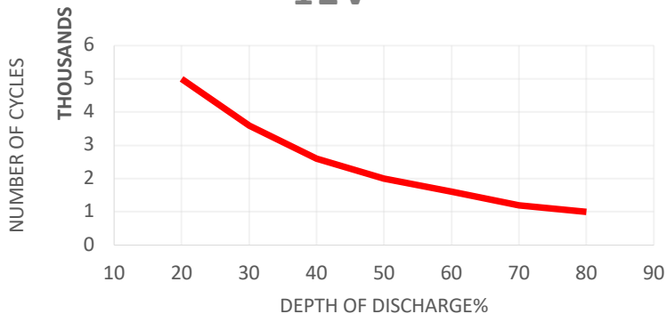
CYCLE LIFE VS DOD FOR 12V
